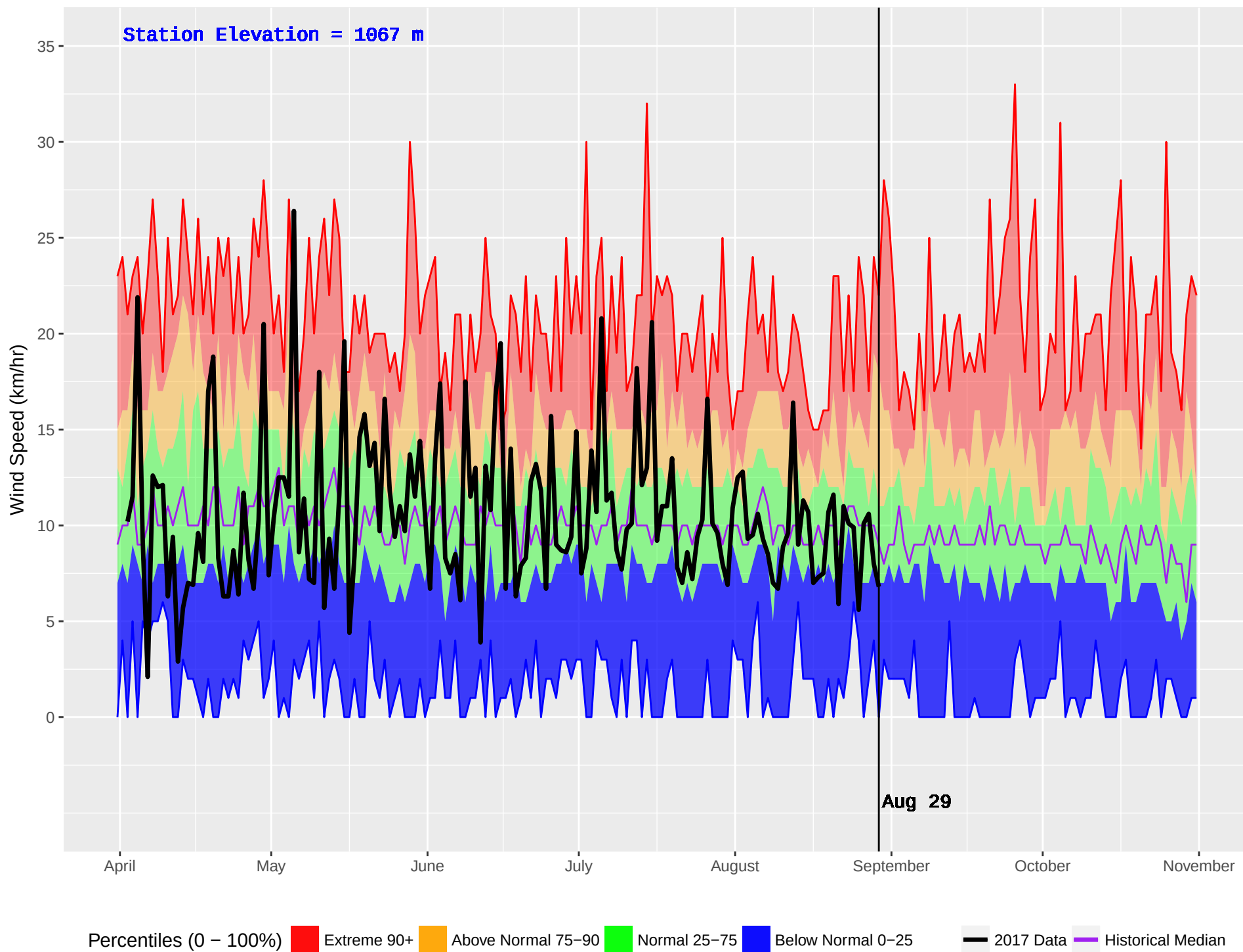
MCCUDDY (334) : Historical (1984–2016) and Current (2017) Noon Wind Speed
